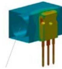
Twall: 50°C Tmax = 72.9°C (Alunit) Tmax = 138.7°C (Rubalit)
