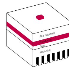
Typical packaging system with multiple layers and different TCEs. Potential risks: Delamination, corrosion, degradation.
