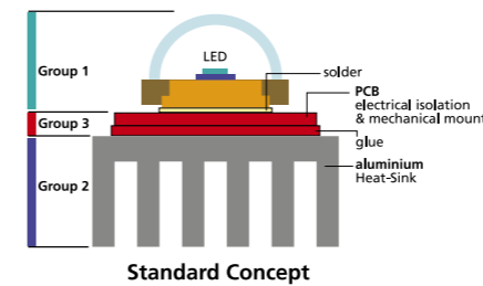
Three groups build a thermal management system and are examined for optimization potential. Why not eliminate block 3?
