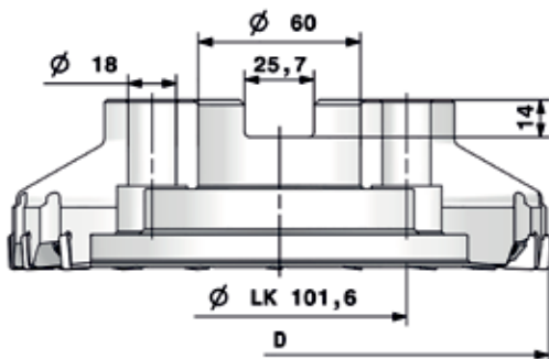
Holding fixture shape C
